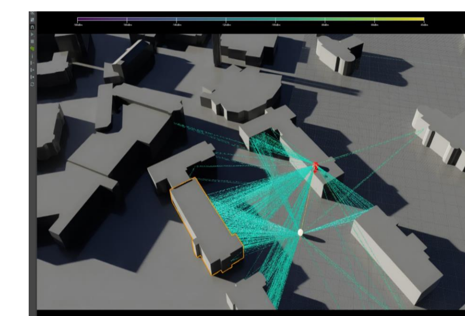
Fig. 11. UW Quad multipath propagation modeled through NVIDIA Omniverse.
