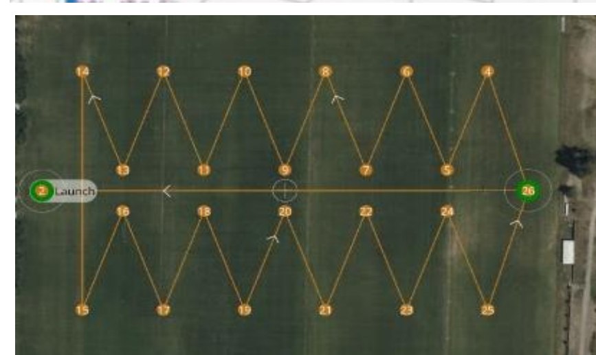
Fig. 5. Grid Flight Path
