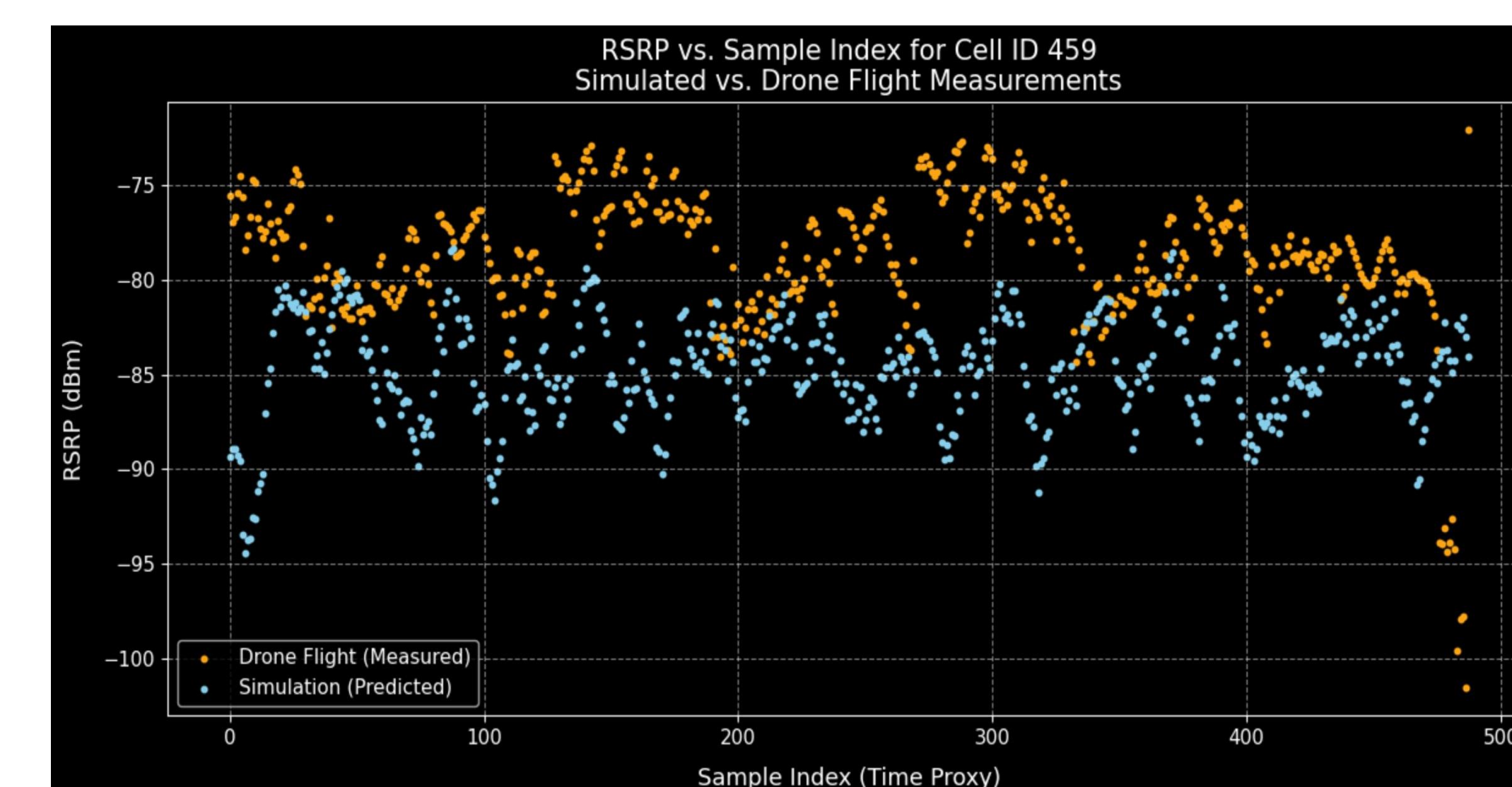
Fig. 13. RSRP Comparison: Simulation VS Real Flight
